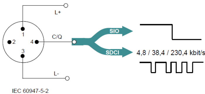
Figure 6-3. SDCI Connection
