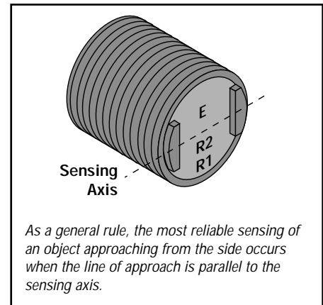
Figure 1. Sensing axis
