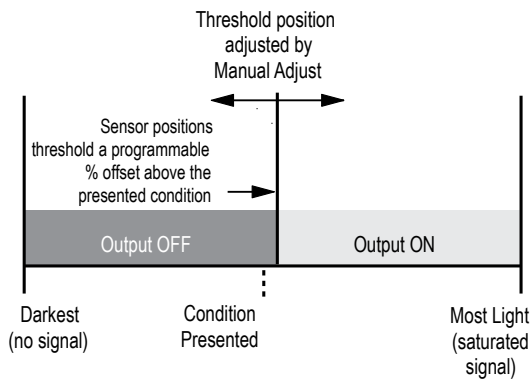
Figure 6. Dark SET (Light Operate shown)
