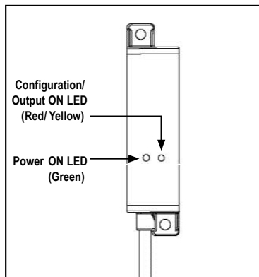
Figure 6. Sensor Features
