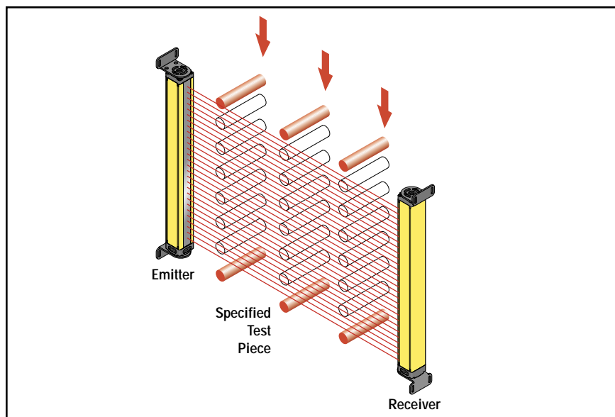
Figure 22. MINI-SCREEN System Trip Test
