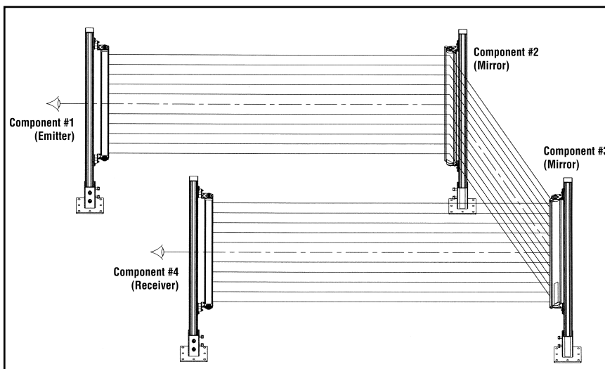
Figure 27. Corner mirror alignment
