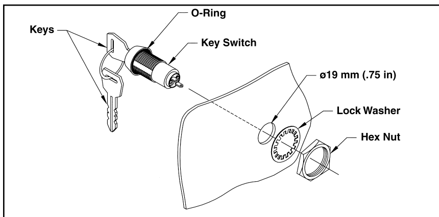
Figure 19. Mounting the MINI-SCREEN key reset switch
