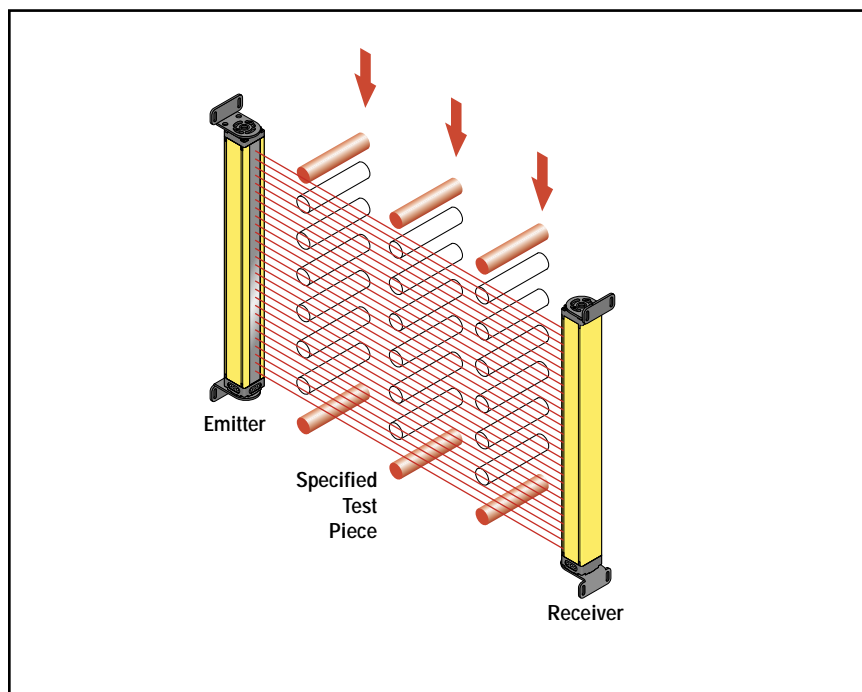
Figure 6-6. MINI-SCREEN trip test
