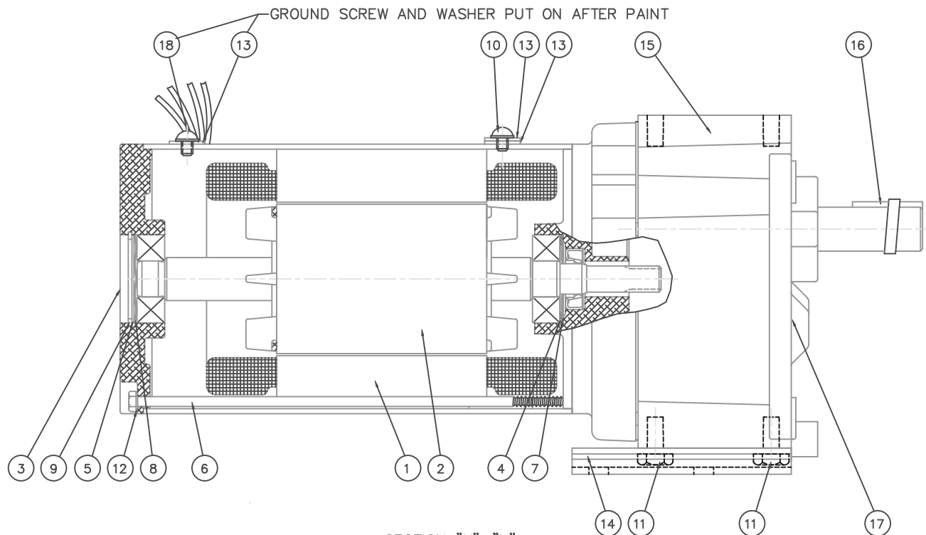
SECTION "X"-"X"
