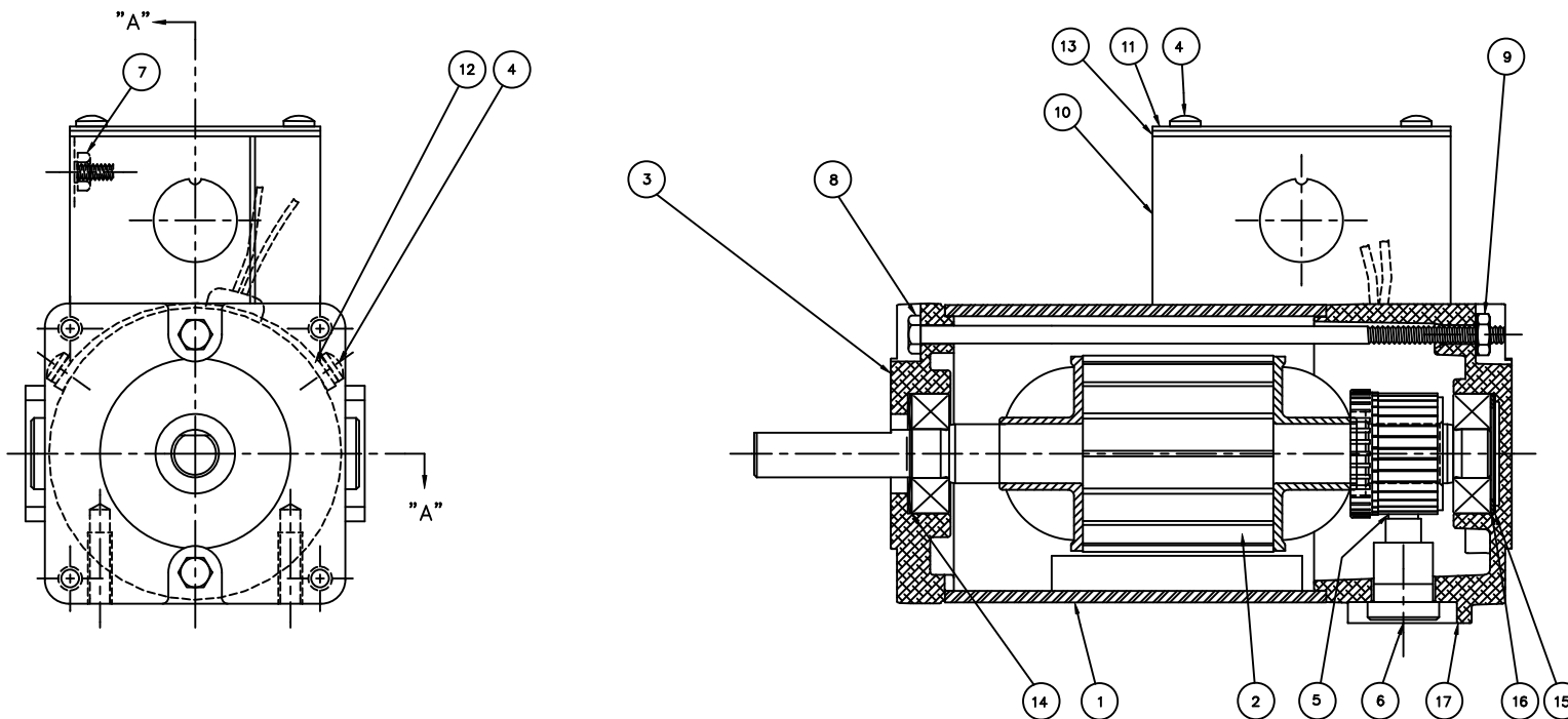
SECTION "A-A"
