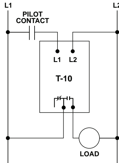
TYPICAL WIRING DIAGRAM FOR MODEL T-10
