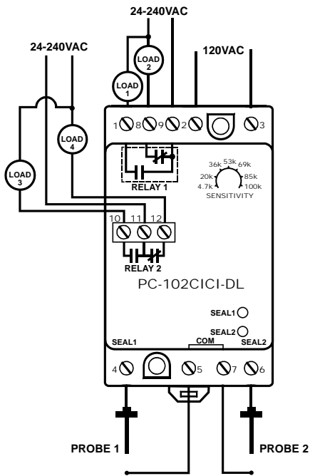
TYPICAL WIRING DIAGRAM FOR PC-102CICI-DL
