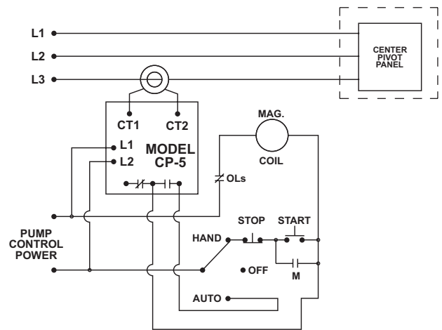
TYPICAL WIRING DIAGRAM FOR MODEL CP-5
