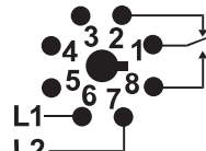
Pin-out 2 (201-200-SP-T-9) (view of socket)
