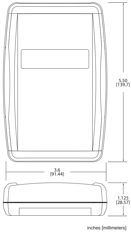
Figure 12 (520-CP, 520-CS)
