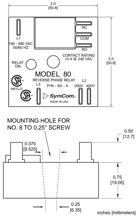
Figure 6 (80)
