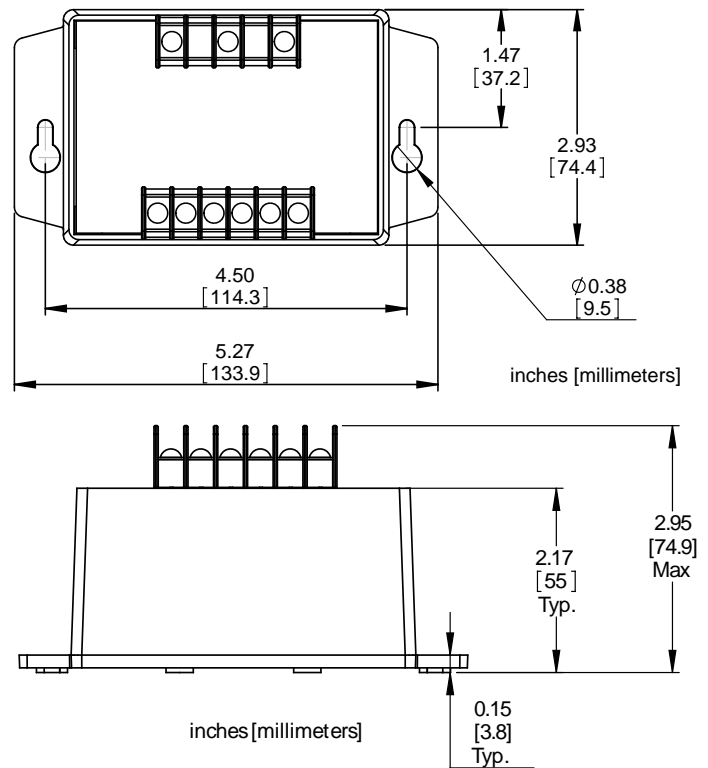
Figure 9 (202, 202-RP, 202-SP)
