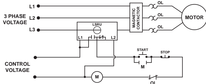
TYPICAL WIRING DIAGRAM FOR MODEL LSRU
