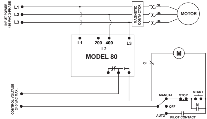
TYPICAL WIRING DIAGRAM FOR MODEL 80 (400VAC)
