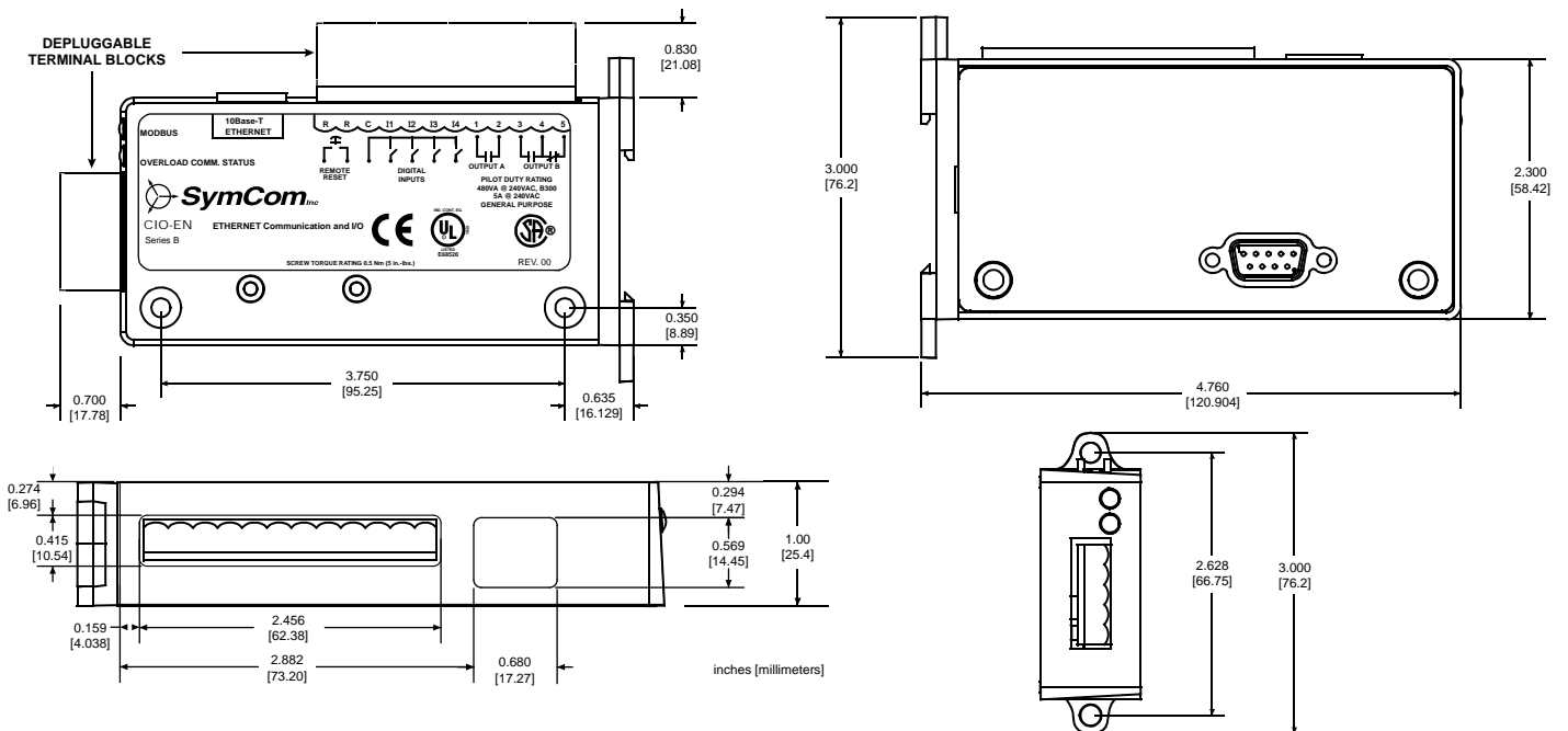
Figure 3 (CIO modules)
