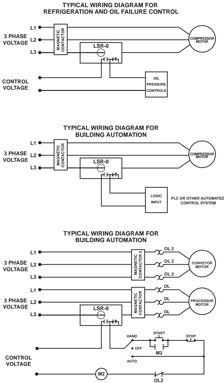
TYPICAL WIRING DIAGRAMS FOR MODEL LSR-0
