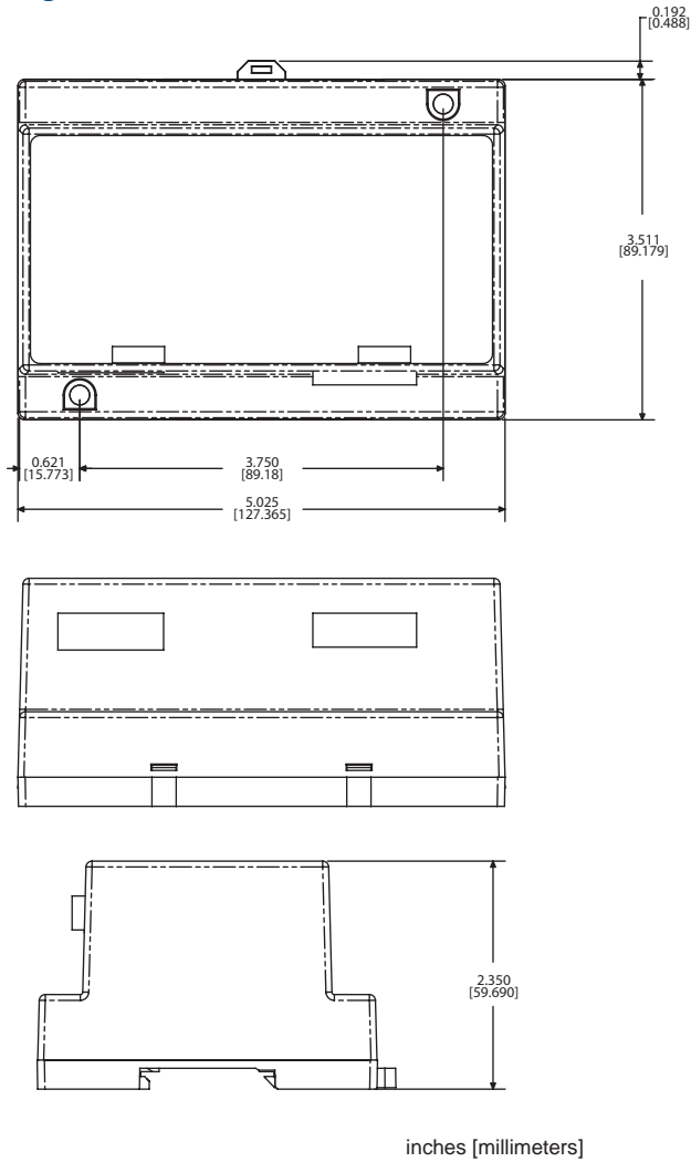
Figure 13 (ISS-105, PC-105)
