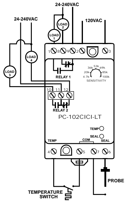
TYPICAL WIRING DIAGRAM FOR PC-102CICI-LT
