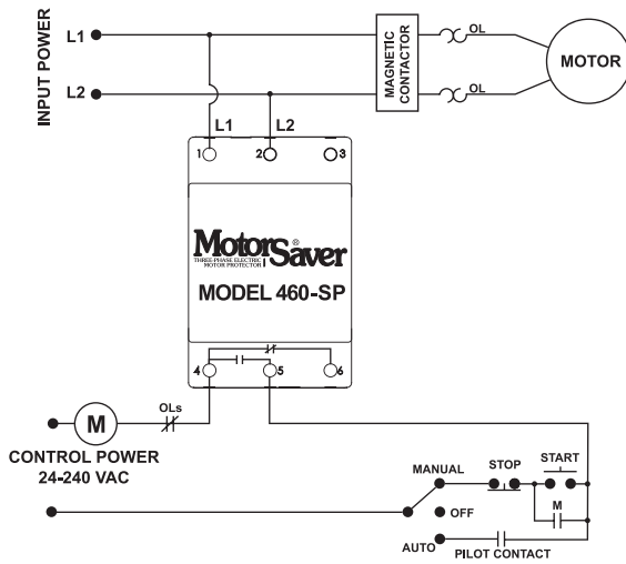
TYPICAL WIRING DIAGRAM FOR MODEL 460-xxx-SP WITH MOTOR CONTROL
