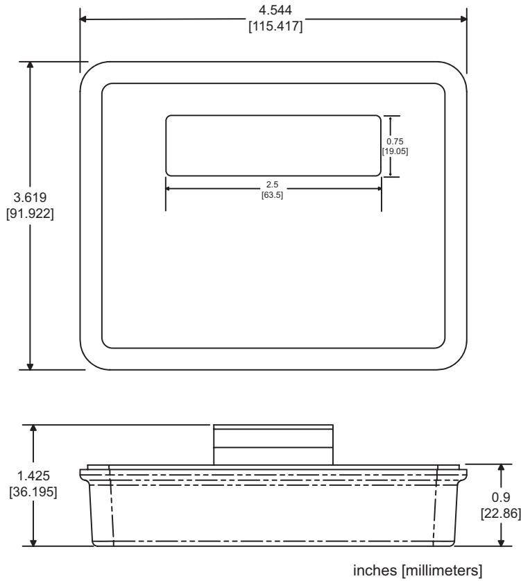
Figure 5 (RM-2000)
