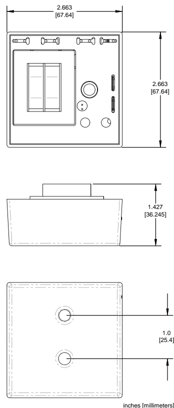
Figure 9 (202, 202-RP, 202-SP)
