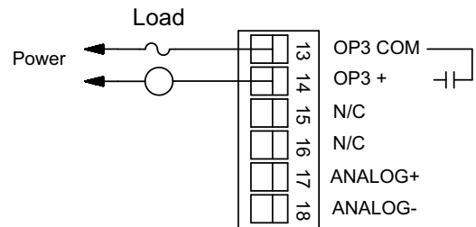
Output 3 - Relay Version
