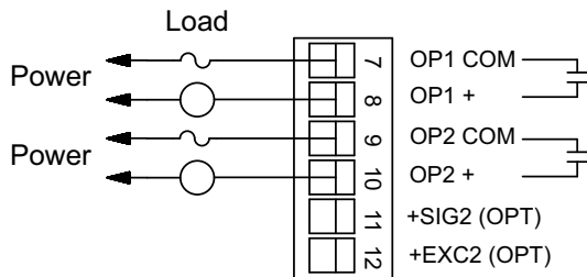
Outputs 1 and 2 - Relay Version
