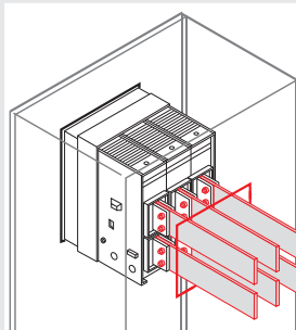
For switchgear with access from the rear
