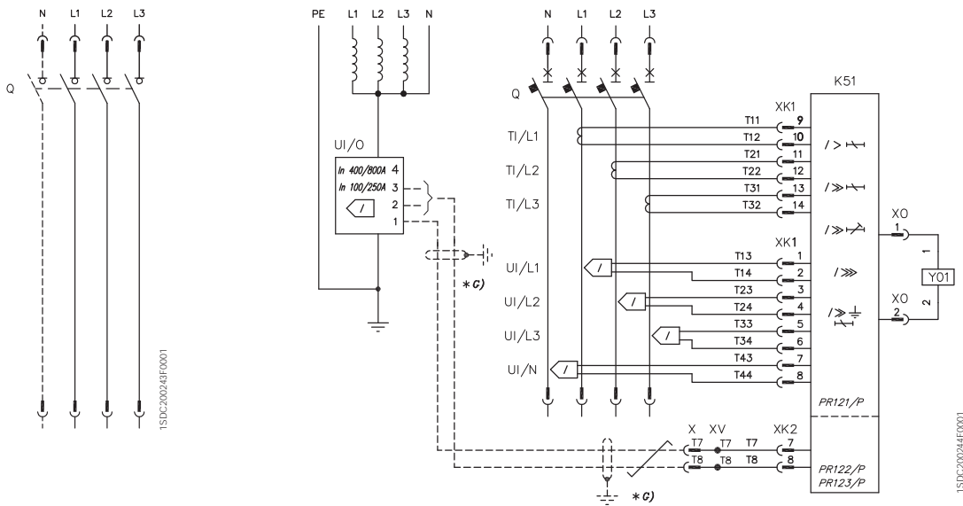
Three- or four-pole switch-disconnector
