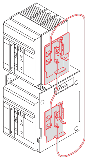
Vertical interlock
