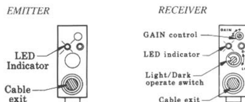
Figure 2. Sensor indicators and adjustments
