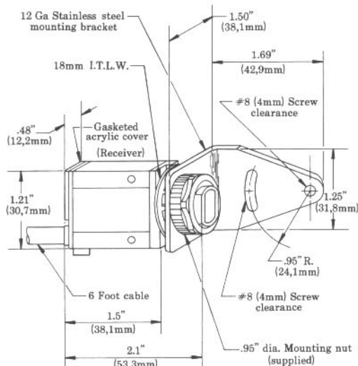
Dimension drawing, DC models SM31EPD & SM31RPD
