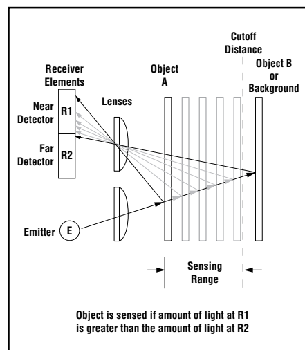
Figure 1. Fixed-field concept
