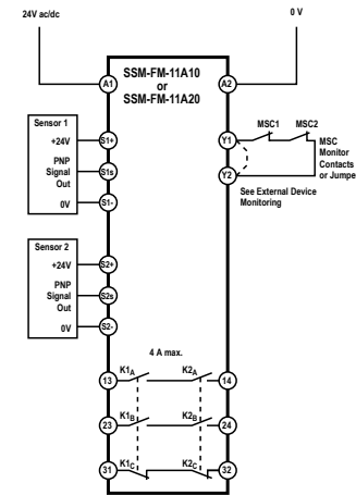
Figure 4. Typical hookup to two sensors
