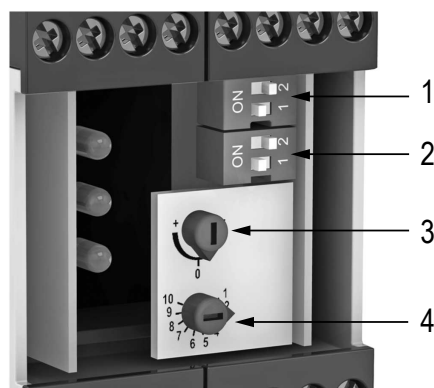
Figure 7. Module adjustments
