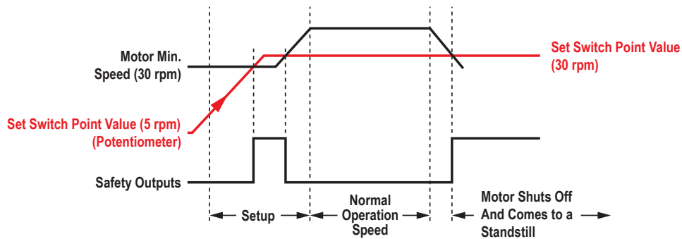
Figure 9. Under-speed Timing
