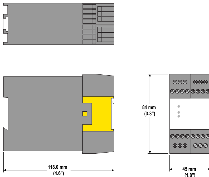
Figure 2. Dimensions—SSM-FM-11A20
