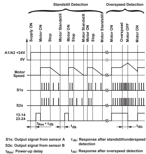
Figure 3. Functional Diagram
