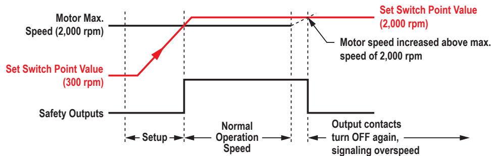
Figure 10. Over-speed Timing
