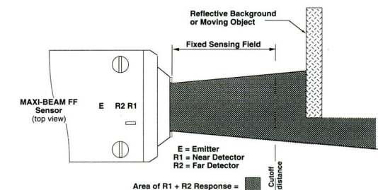
Figure 6. Object beyond cutoff - solution
