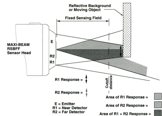
Figure 5. Object beyond cutoff - problem
