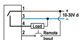
4-Pin PNP Models
