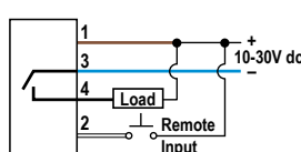
4-Pin NPN Models
