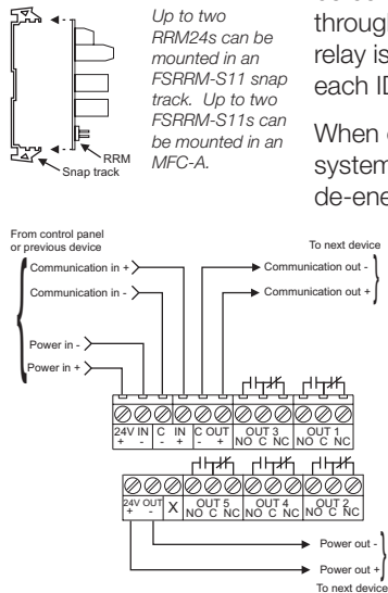
The Remote Relay Module mounts on a plastic track inside an MFC-A cabinet.
