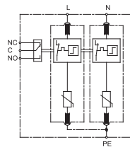
SCHEMATIC 5
