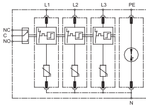
SCHEMATIC 6
