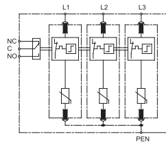
SCHEMATIC 6
