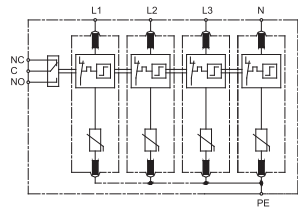
SCHEMATIC 4
