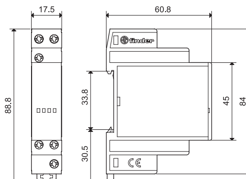
13.31/13.91 Screw terminal
