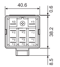
062.07 with relay
