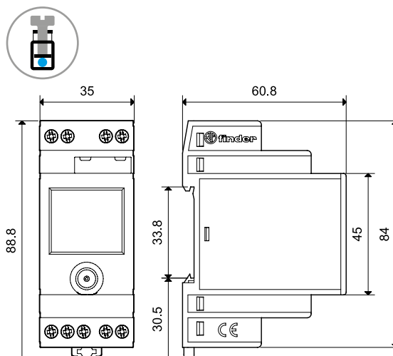
11.91 Screw terminal
