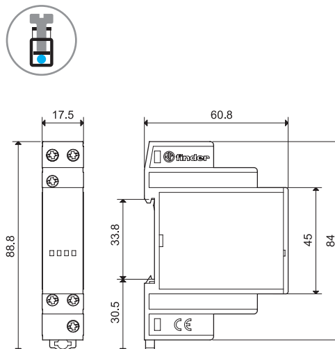
13.11 Screw terminal
