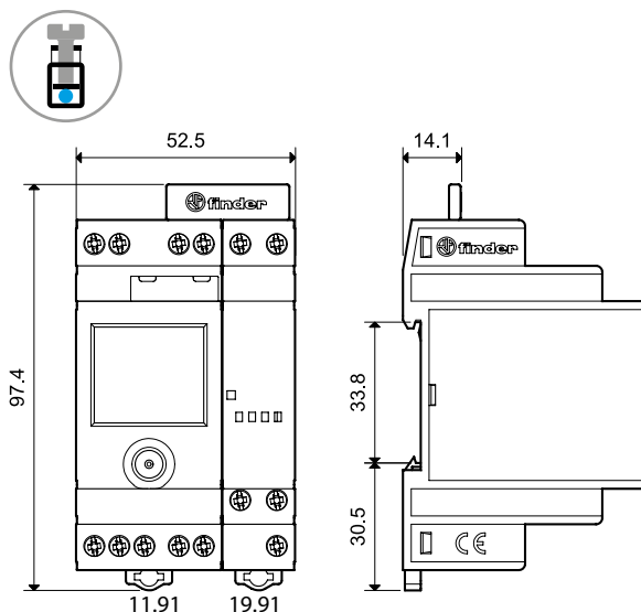
11.91 + 19.91 power module Screw terminal
