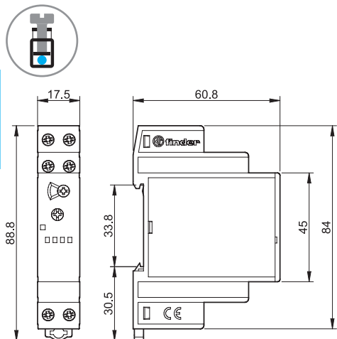
13.61 Screw terminal
