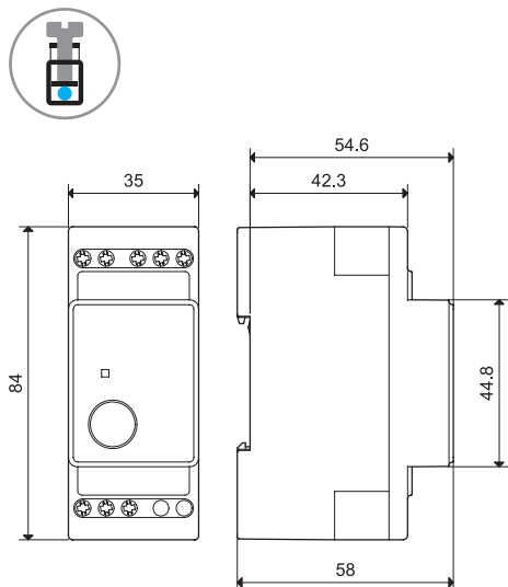
13.12 Screw terminal
