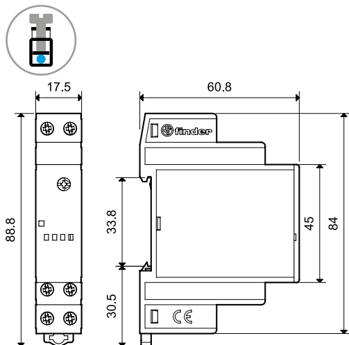
11.31 Screw terminal
