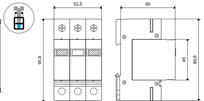
Type 7P.26.9.420.1020 Screw terminal
