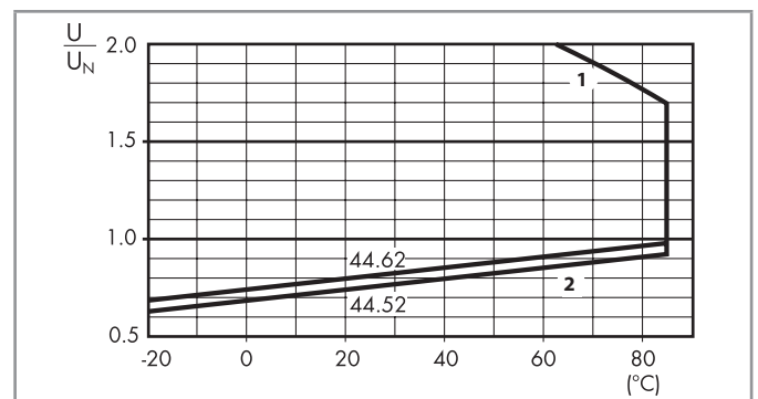
R 44 - DC coil operating range v ambient temperature
