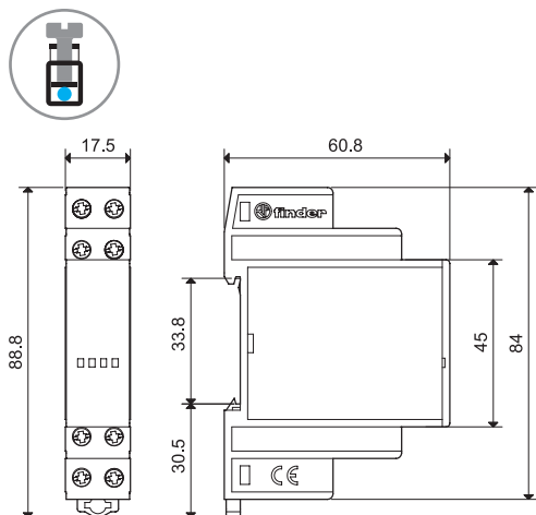
13.61 Screw terminal
