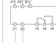
Wiring diagram (with control signal)
