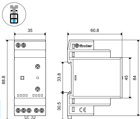
11.41 Screw terminal
