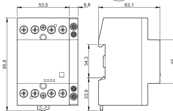
Type 022.63/022.65 Screw terminal
