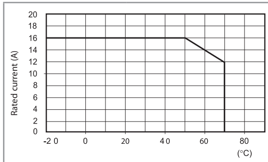
L 97 - Rated current vs ambient temperature
