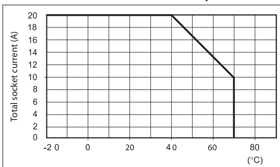
L 95 - Total socket current vs ambient temperature
