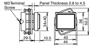
ø30 EB3P-LUN4 Terminal Cover: APN-PVL (sold separately)
