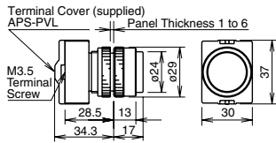
ø22 EB3P-LHW1/EB3P-LHW2/EB3P-LHW4 Terminal cover attached.
