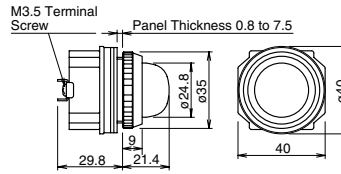
ø30 EB3P-LAD Terminal Cover: APD-PVL (sold separately)
