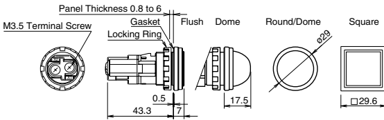
ø22 EB3P-LHW1/EB3P-LHW2/EB3P-LHW4 Terminal cover attached.
