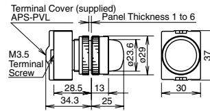
ø22 EB3P-LLW1/EB3P-LLW2/EB3P-LLW3 Terminal cover attached.
