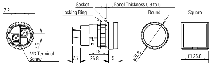
ø22 EB3P-LLW1/EB3P-LLW2/EB3P-LLW3 Terminal cover attached.
