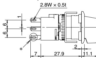
Lever Operator Solder/Tab Terminal
