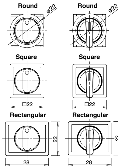
Knob Operator Knob Operator Lever Operator
