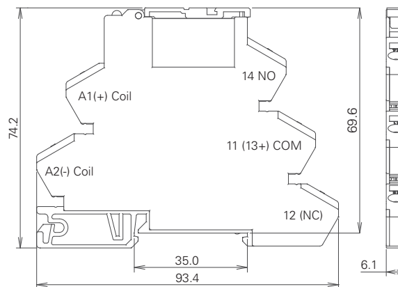
RV8H-S Spring Clamp Terminal (mm)
