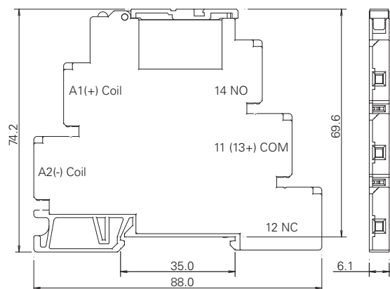
RV8H-L Screw Terminal (mm)
