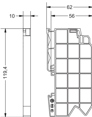
End block
