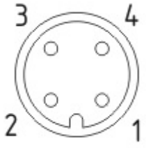
Contact arrangement
