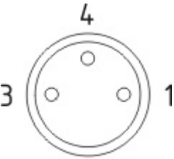
Contact arrangement
