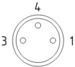
Contact arrangement
