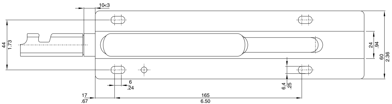
B4pS actuator for hand operated locking
