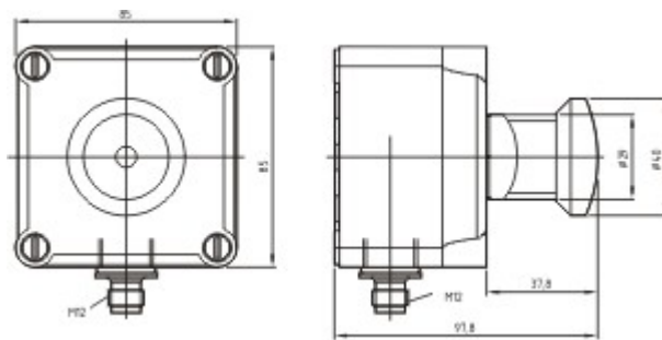
Dimensional drawing (basic component)
