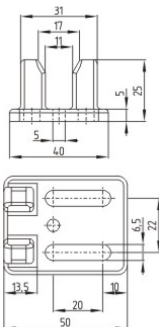
Dimensional drawing (basic component)
