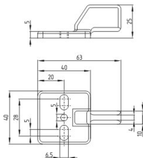
Dimensional drawing (basic component)
