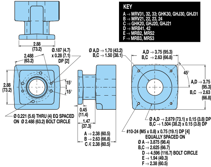
BOTTOM MOUNT
