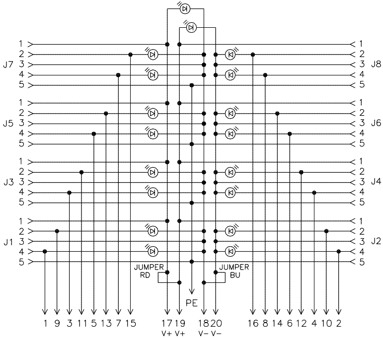
WIRING DIAGRAM (FACTORY SETTING)
