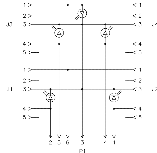
WIRING DIAGRAM
