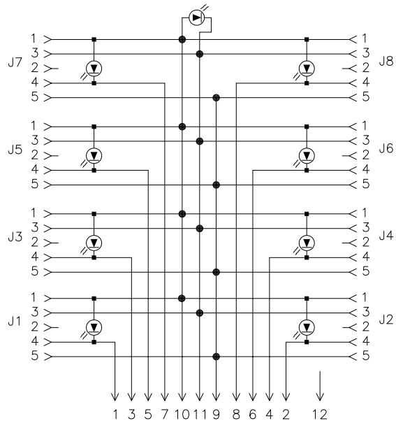
P1 WIRING DIAGRAM
