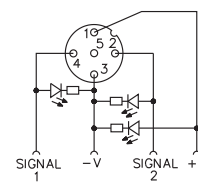
(PNP LED Version) 2 Signals Per Port
