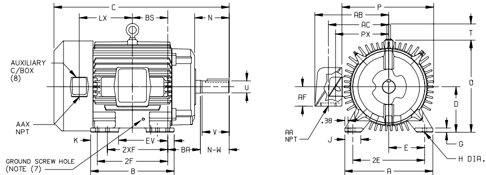
DIMENSIONS ARE IN INCHES
