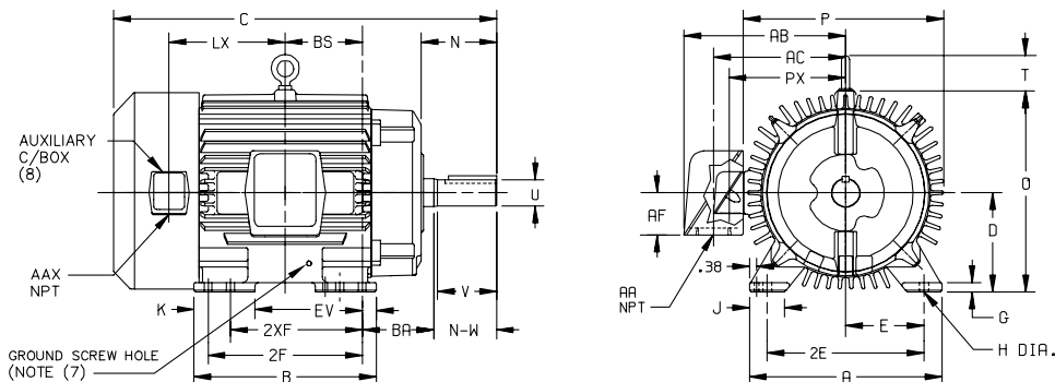
DIMENSIONS ARE IN INCHES
