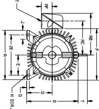
DIMENSIONS ARE IN INCHES: SEE SHEET 2 FOR DIMENSIONS IN MILLIMETERS
